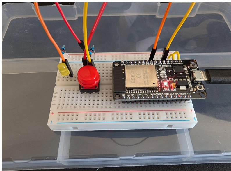
Figure 2: This experiment allowed notifications to be displayed with every push of the button. The LED attached would also light up to indicate that the button was indeed pushed.
