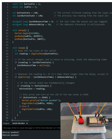
Figure 2: This experiment allowed notifications to be displayed with every push of the button. The LED attached would also light up to indicate that the button was indeed pushed.
